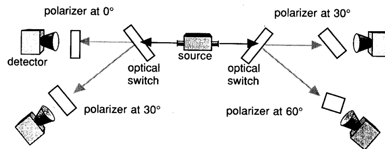
Figure 1.4 Aspect's Experiment
